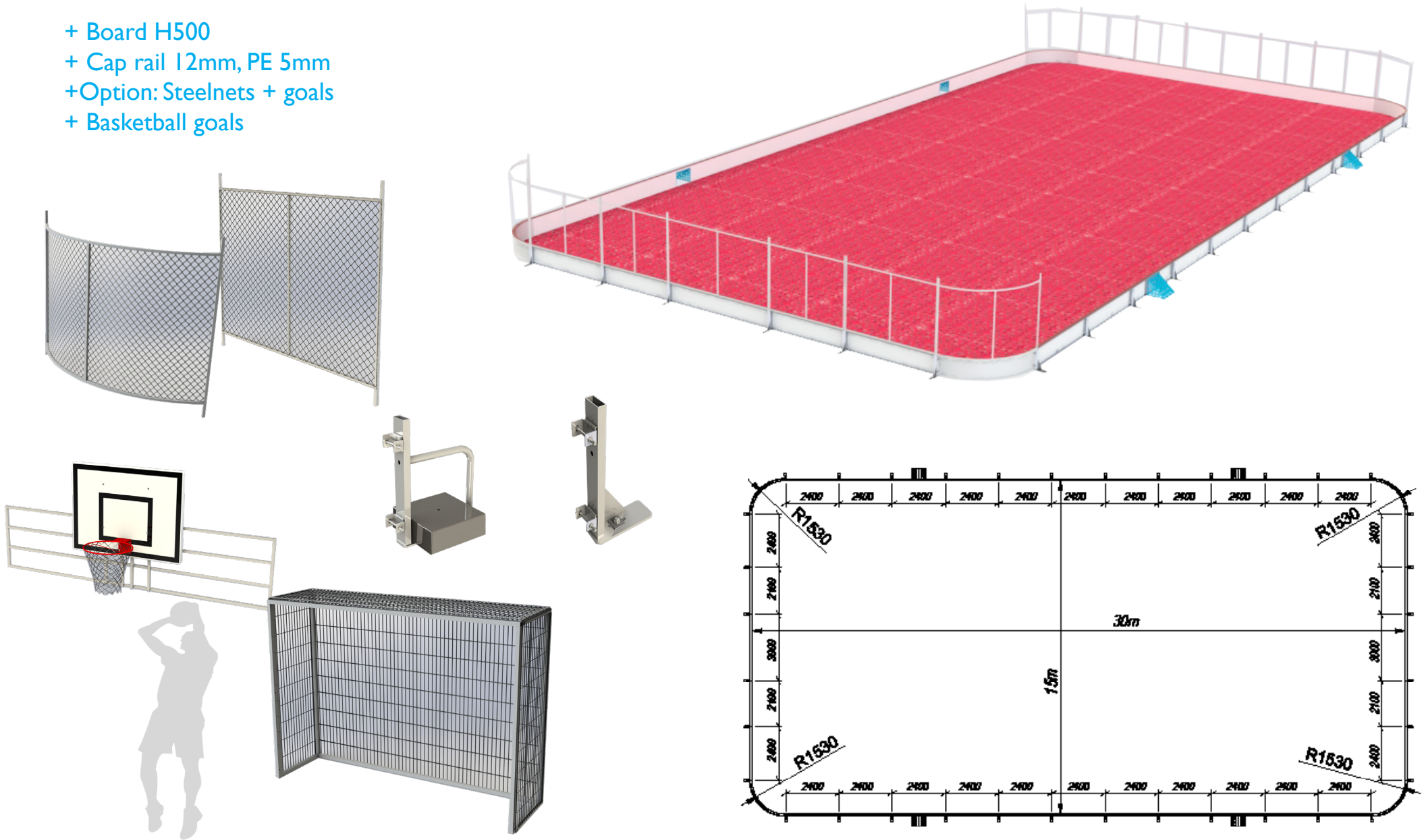
Rink layout 15m x 30m
