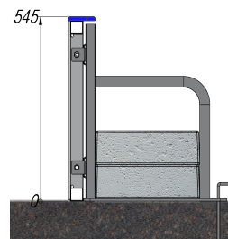
Cut view
