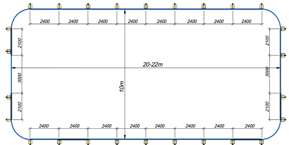
Rink Layout 10m x 20-22m
